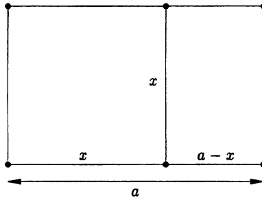
Figura 15: Rectangle auri
